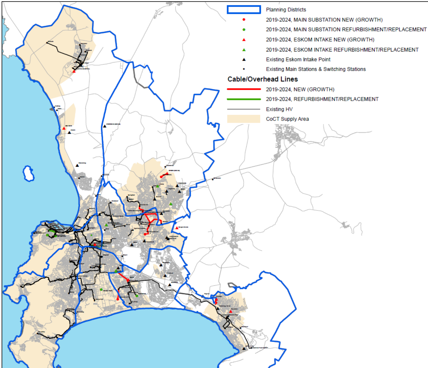
Figure 38: Proposed electrical infrastructure projects in Cape Town
