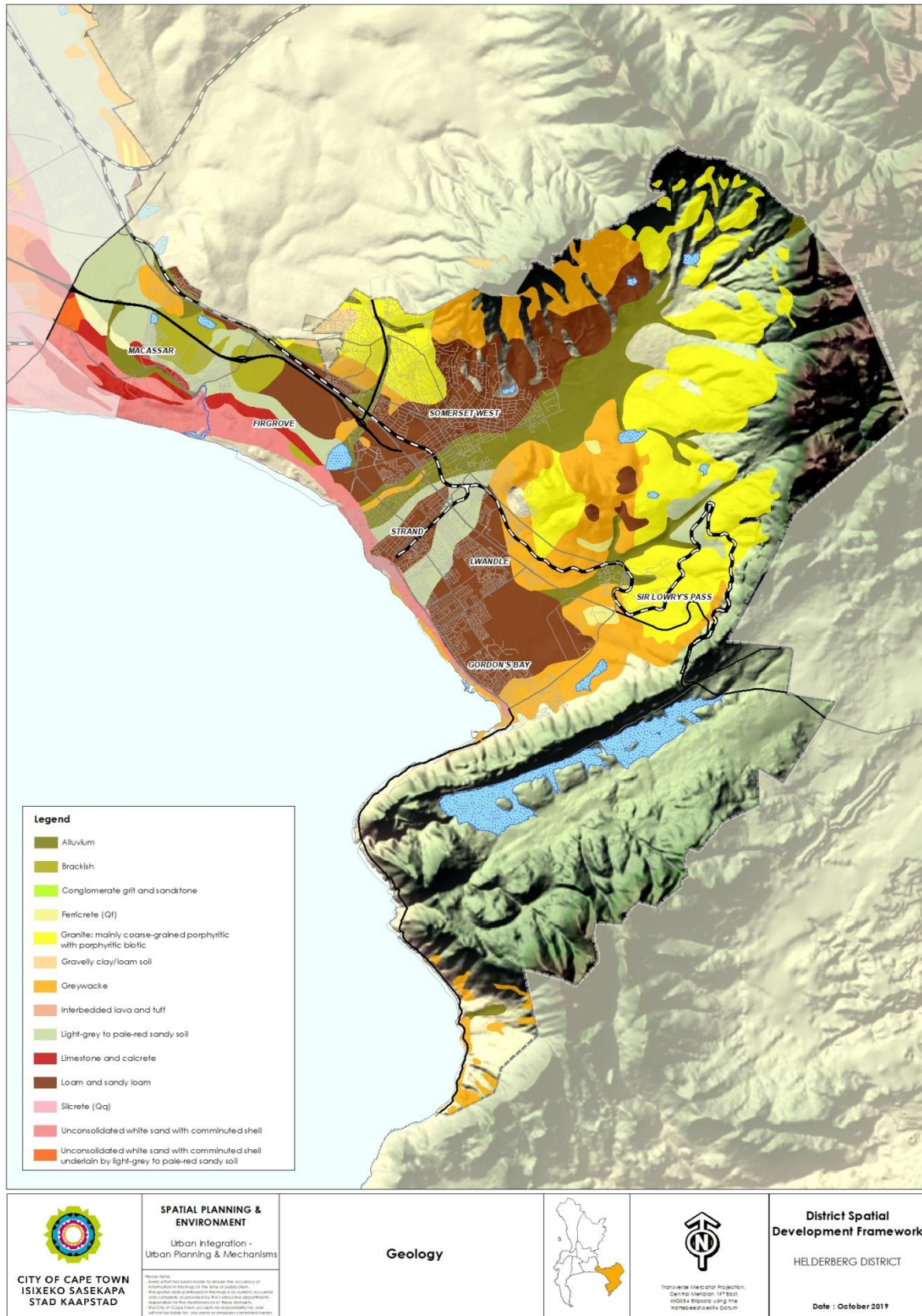
Figure 17: Underlying geology of the Helderberg District
