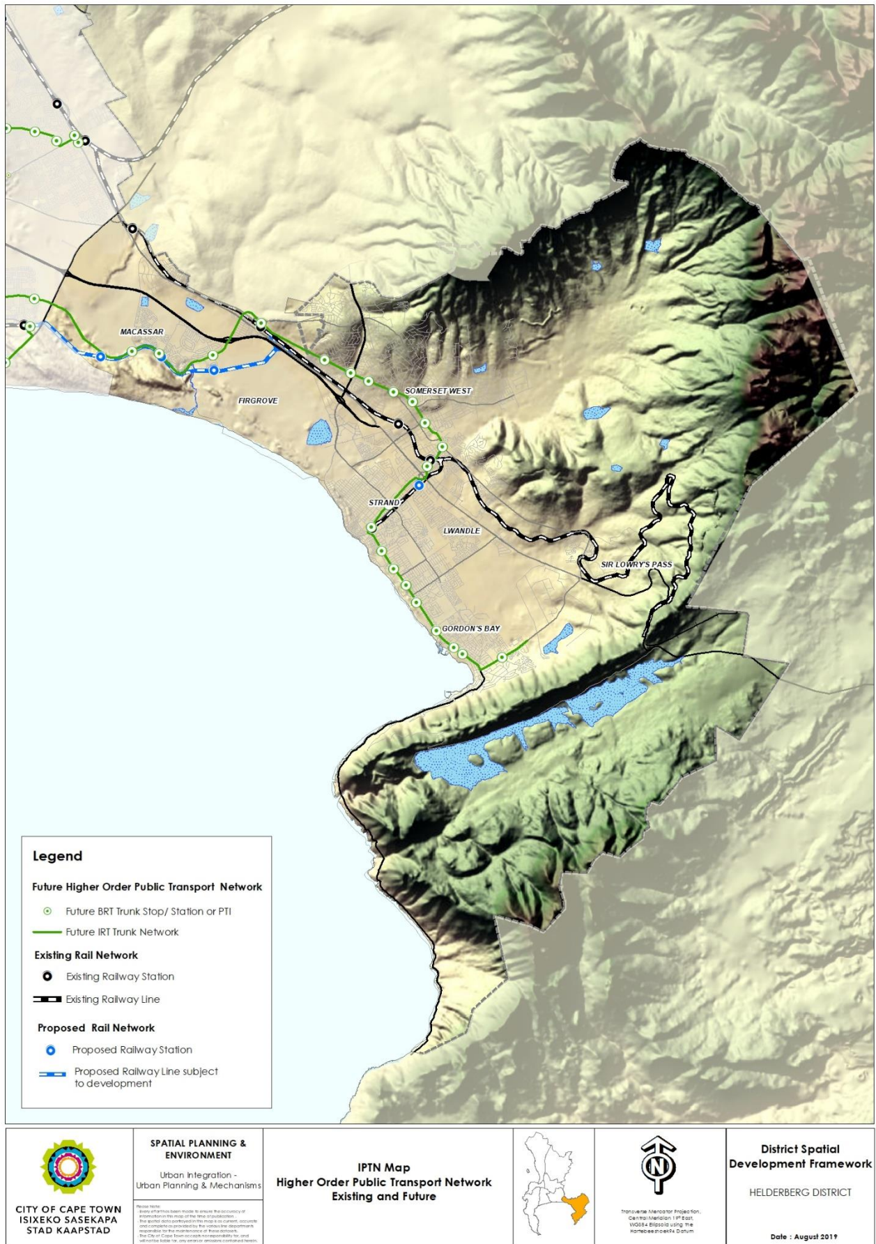
Figure 26: Existing and future high-order public transport services in the Helderberg District (IPTN, 2032)
